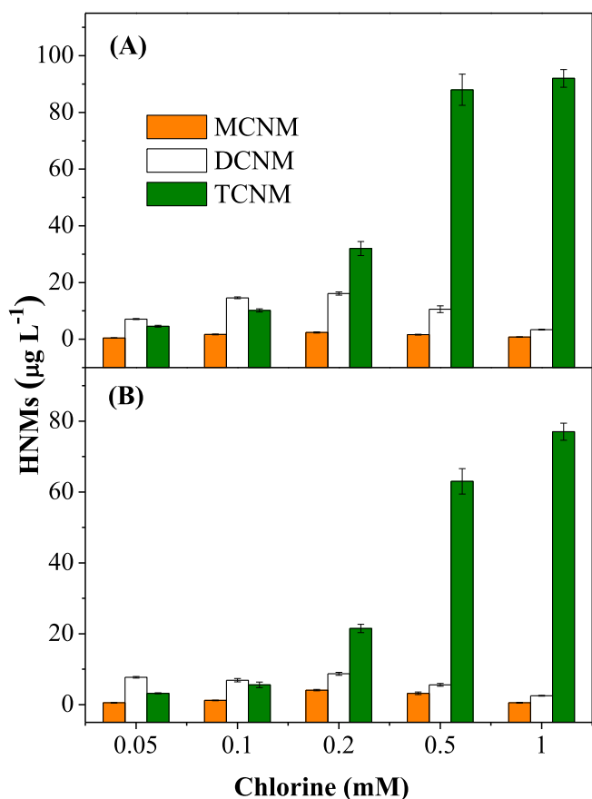
Fig. 3. Effect of initial chlorine concentration on HNMs formation from RNTD (A) and NZTD (B). Experimental conditions: [RNTD \text{ or } NZTD]_0 = 10 \mu M , pH 7.0, reaction time = 24 h. Error bars represent the 95% confidence interval.
