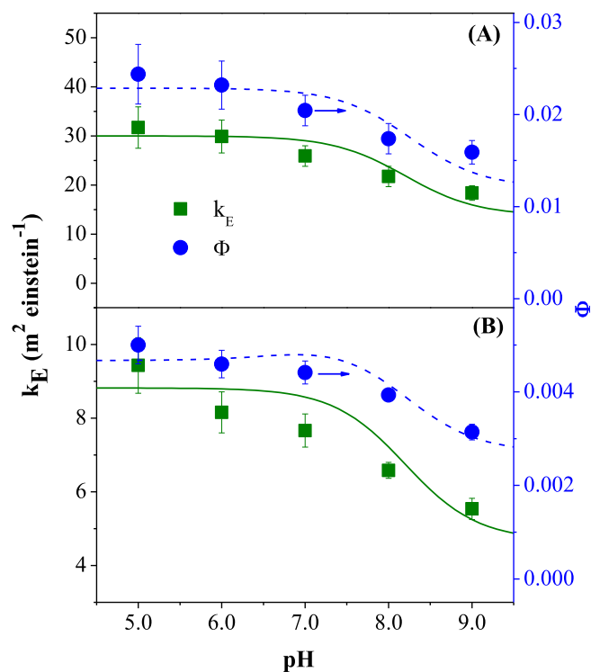
Fig. 2. Apparent photon fluence-based rate constants ( k_E ) and quantum yields ( \Phi ) of RNTD (A) and NZTD (B) as a function of pH. Experimental conditions: [RNTD or NZTD] 0 = 10 μM, UV fluence rate = 2.1 mW cm -2 (or photon fluence rate = 446.8 E m -2 s -1 ). Symbols and curves (solid and dashed) represent experimental data and model-fitting results, respectively. Error bars represent the 95% confidence interval of triplicate experiments.
