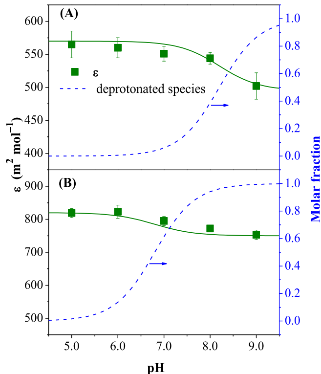
Fig. 1. Molar absorption coefficients ( \epsilon ) at 254 nm and fraction of deprotonated species of RNTD (A) and NZTD (B) as a function of pH. Experimental conditions: [RNTD or NZTD] 0 = 10 μM, UV fluence rate = 2.1 mW cm -2 . Symbols and solid curves represent experimental data and model-fitting results, respectively. Dashed curves represent the fractions of deprotonated RNTD and NZTD. Error bars represent the 95% confidence interval of triplicate experiments.
