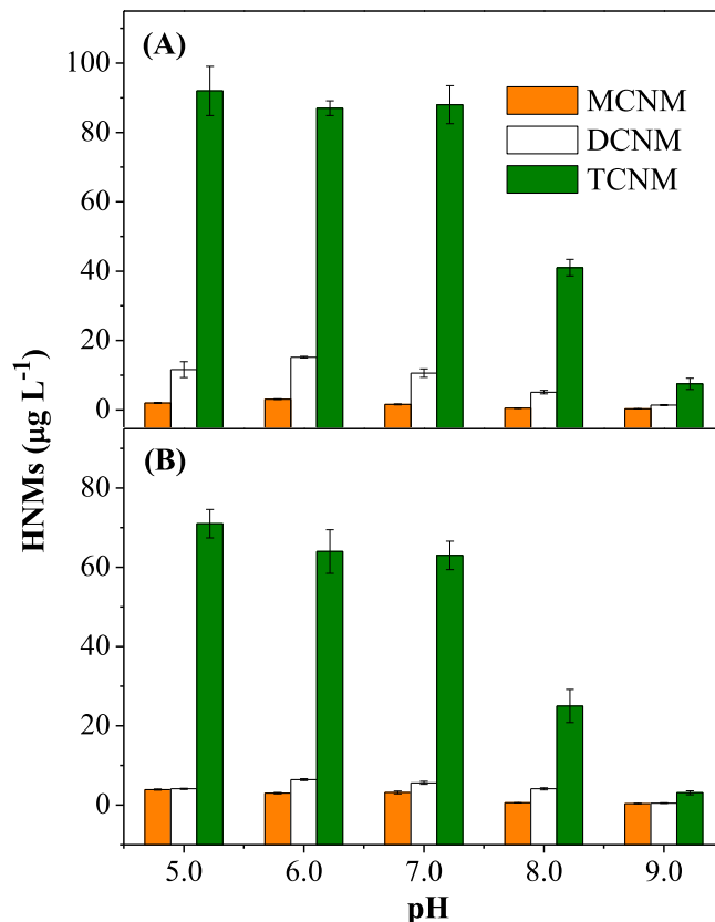
Fig. 4. Effect of pH on HNMs formation during chlorination of RNTD (A) and NZTD (B). Experimental conditions: [RNTD \text{ or } NZTD]_0 = 10 \mu M , [\text{chlorine}]_0 = 0.5 \text{ mM} , reaction time = 24 h. Error bars represent the 95% confidence interval.
