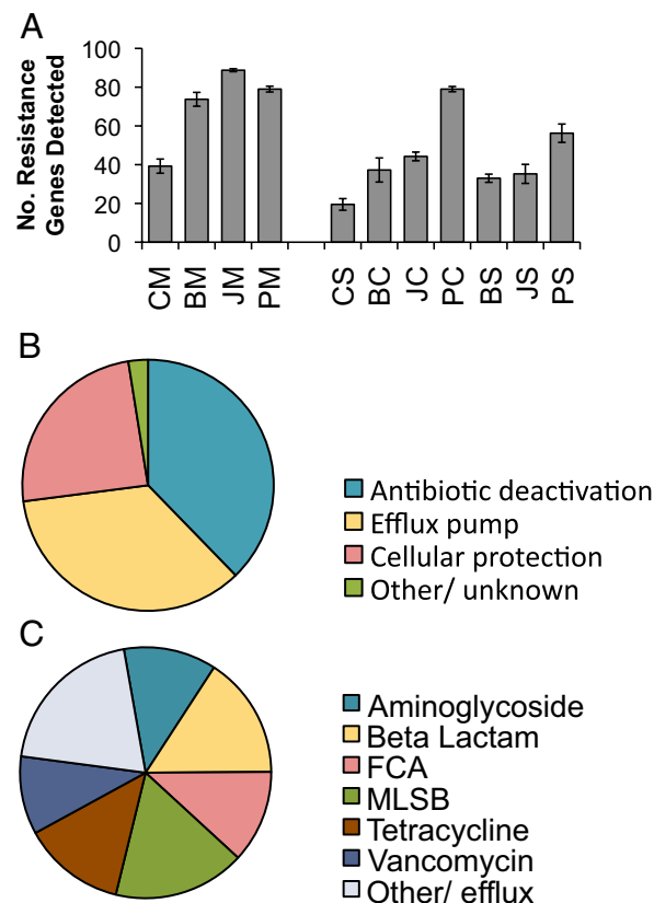
Fig. 1. Antibiotic resistance gene detection statistics. Sample names are abbreviated with two letters representing location and sample type: first C, B, J, and P (control, Beijing, Jiaying, and Putian, respectively) and second M, C, and S [manure, compost, and soil (with compost amendment), respectively]. Because many resistance genes were targeted with multiple primers, if multiple primer sets detected the same gene, this was only counted as detection of a single unique resistance gene. (A) Average number of unique resistance genes detected in each sample. Error bars represent SEM of four field replicates. The resistance genes detected in all samples were classified based on (B) the mechanism of resistance, and (C) the antibiotic to which they confer resistance. FCA, fluoroquinolone, quinolone, florfenicol, chloramphenicol, and amphenicol resistance genes; MLSb, Macrolide-Lincosamide-Streptogramin B resistance.
