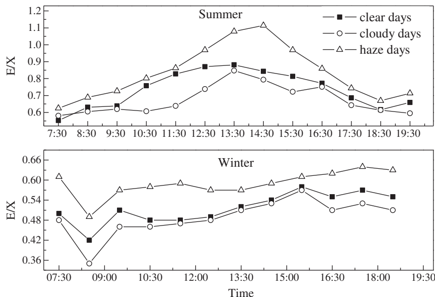
Fig. 2. The average diurnal variations of ethylbenzene/ m,p -xylene (E/X) under three typical days in summer and winter.
