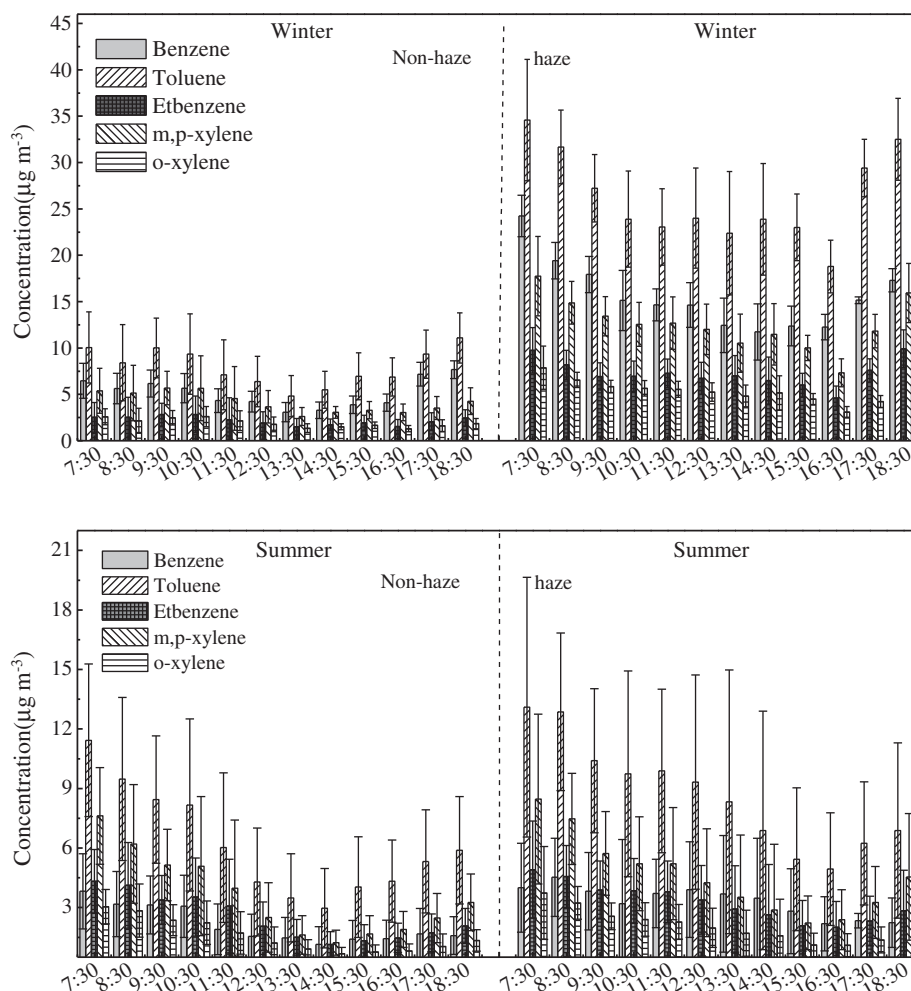
Fig. 1. Average diurnal variations of BTEX under haze days and non-haze days in winter and summer.
