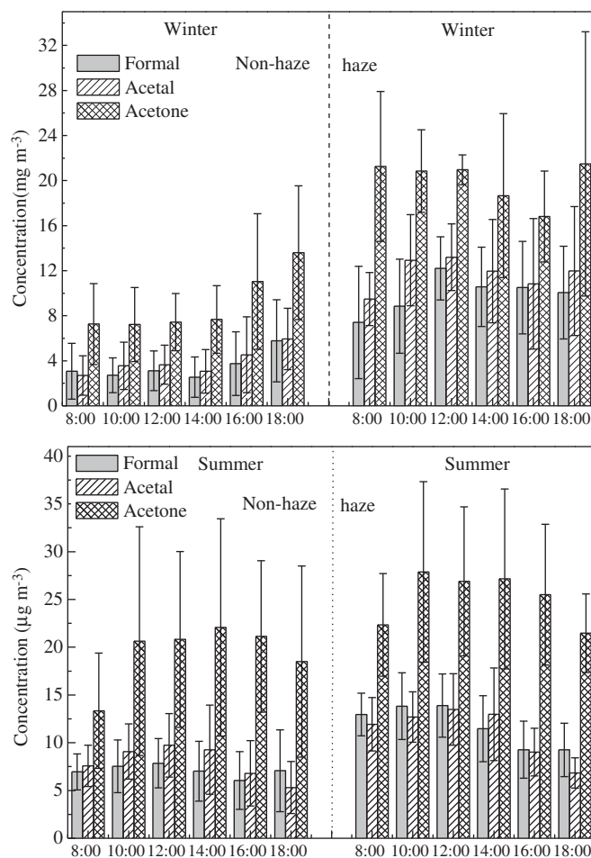
Fig. 3. Average diurnal variations of three principle carbonyls under haze days and non-haze days in winter and summer.
